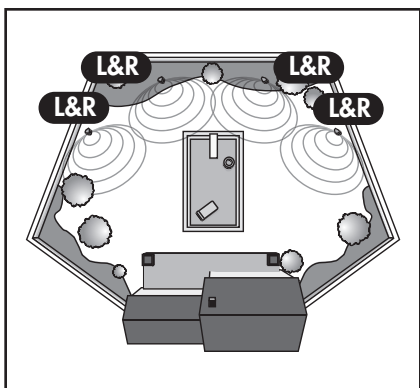
Figure 3. Distributed multi-speaker 'Left & Right' stereo from a single speaker
