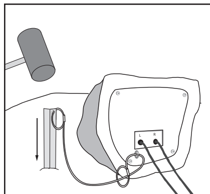
Figure 7d. Drive the stake into the ground.
